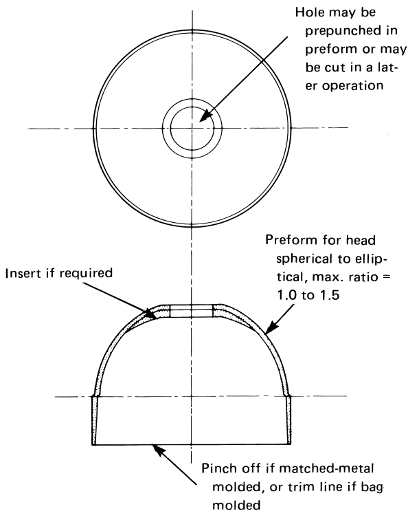
Figure RF-610.1 Fiber Preform and Insert for Centrifugally Cast Vessel
