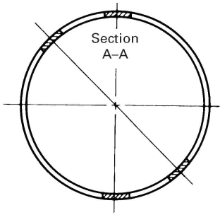
(a) Cut Samples From Section of Vessel or From Sample Section
