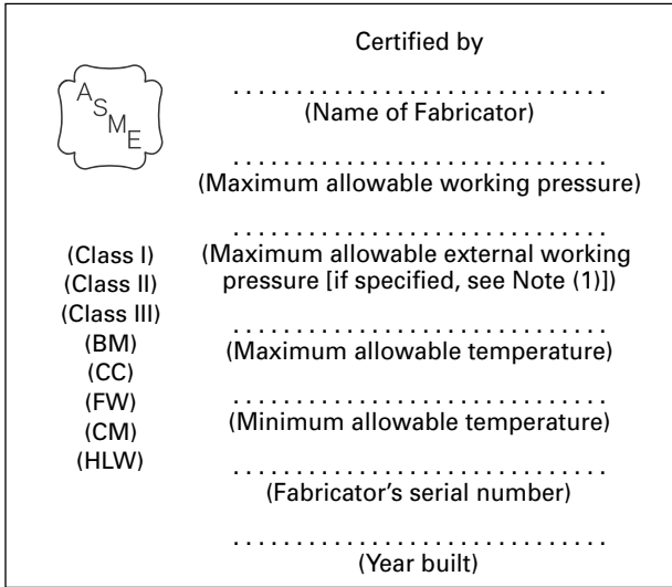
Figure RS-132.1 Form of Stamping and Marking
