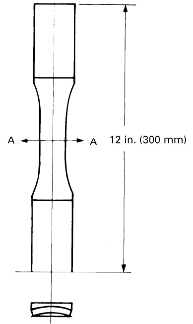
(b) Longitudinal Tensile Test Samples Cut From Vessel Side Wall [Note (1)]
